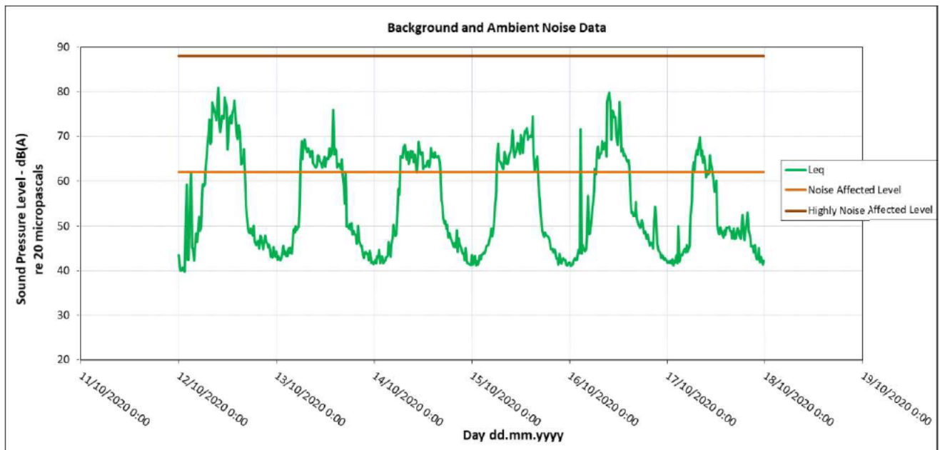
Figure 12: Logger 1 monitoring result 12/10-18/10
