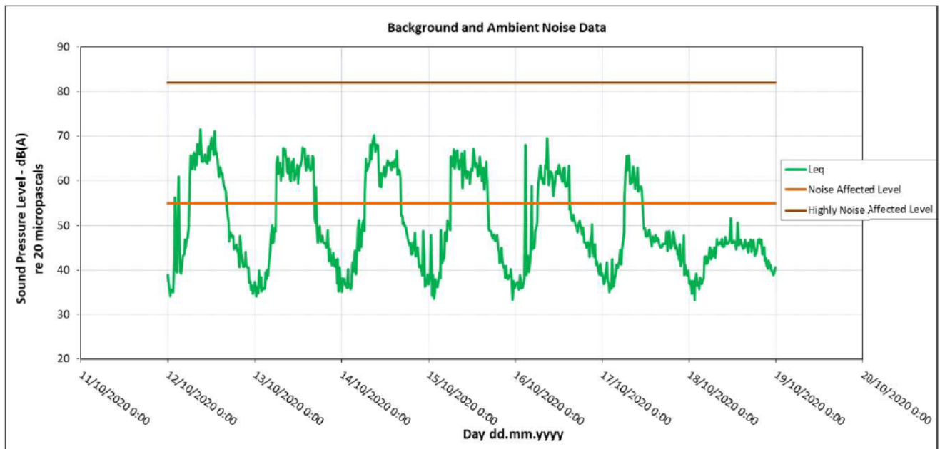
Figure 8: Logger 1 monitoring result 12/10-18/10
