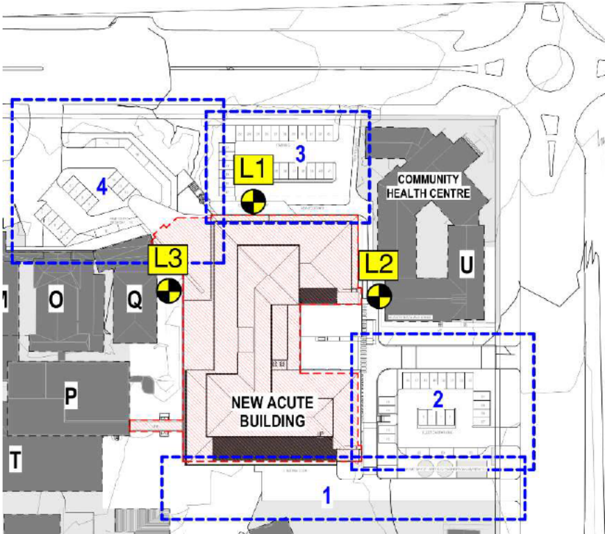
Figure 4: On site location of noise monitors
