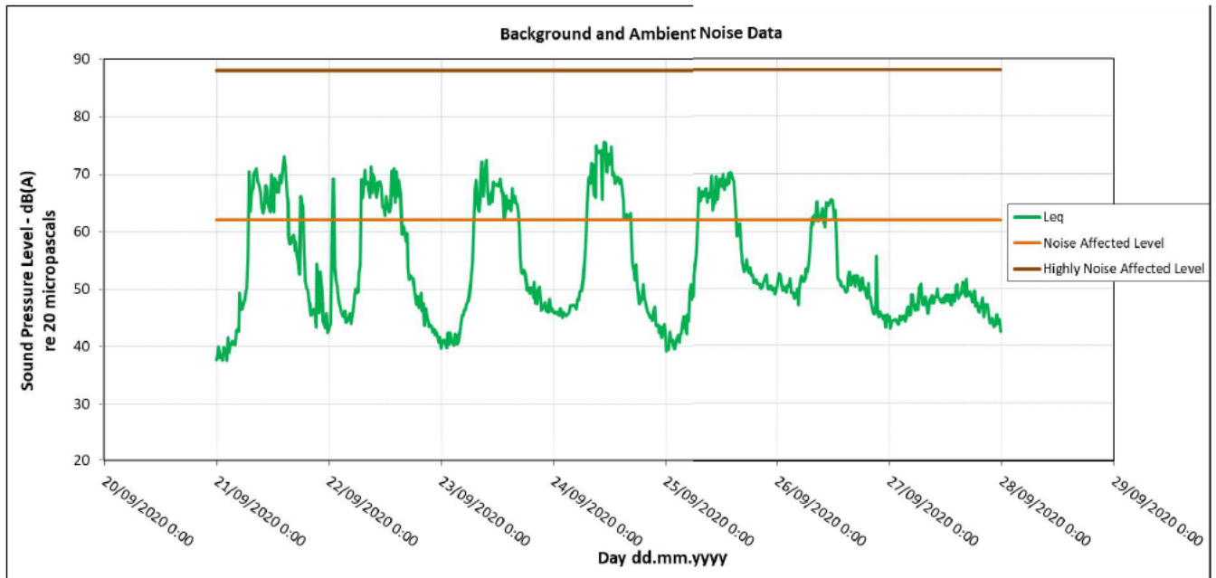
Figure 9: Logger 1 monitoring result 21/09-27/09
