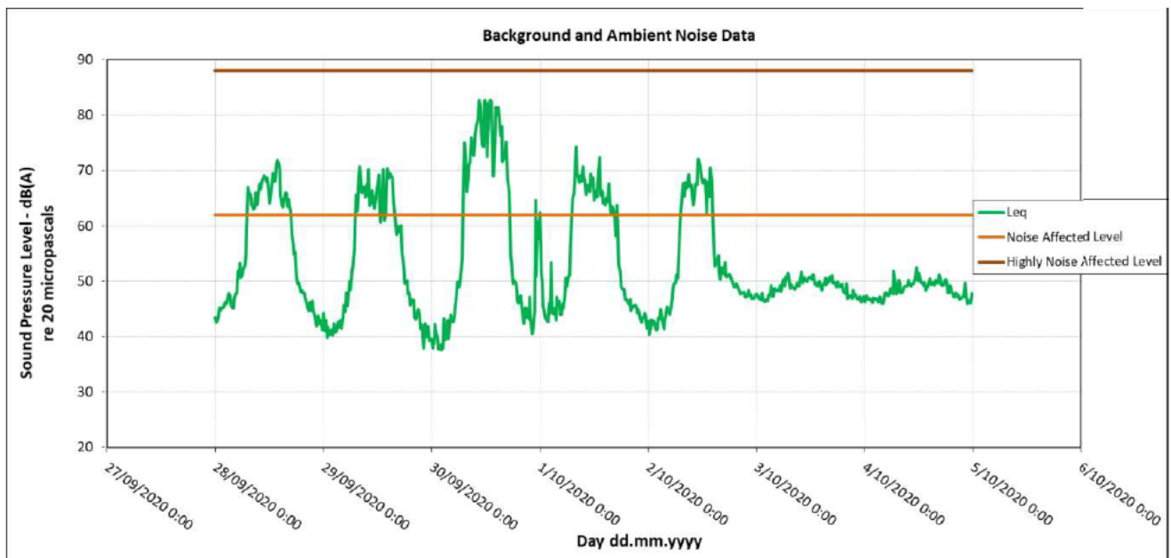
Figure 10: Logger 1 monitoring result 28/09-04/10
