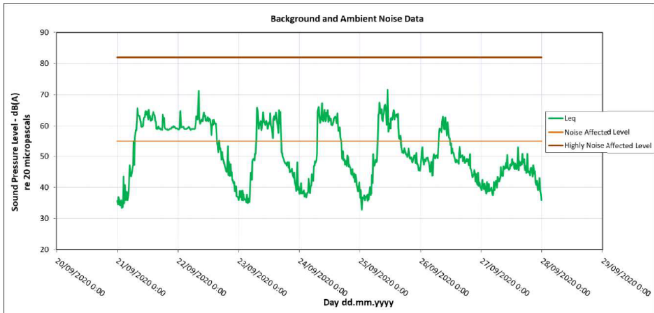
Figure 5: Logger 2 monitoring result 21/09-27/09
