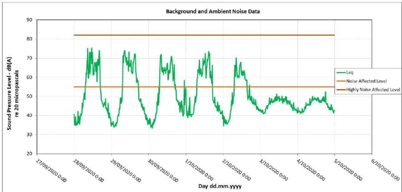
Figure 6: Logger 2 monitoring result 28/09-04/10
